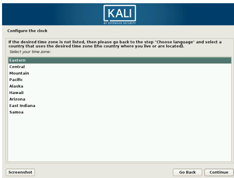
Figure 4.7 Timezone Selection
